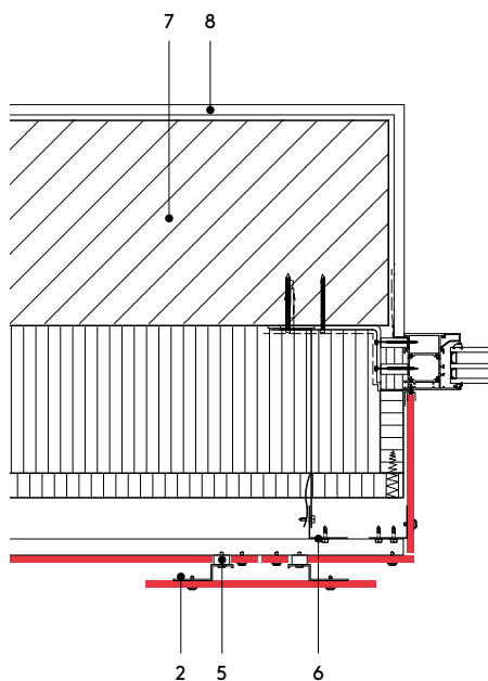
HORIZONTAL SECTION 1:10
