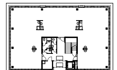
FIRST FLOOR 1:500
