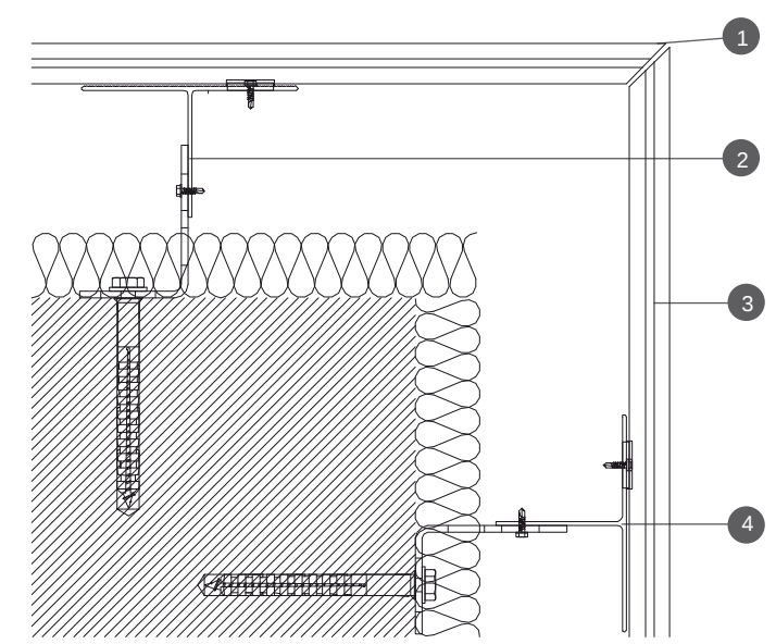
Detalle Esquina a inglete Miter Corner Detail
