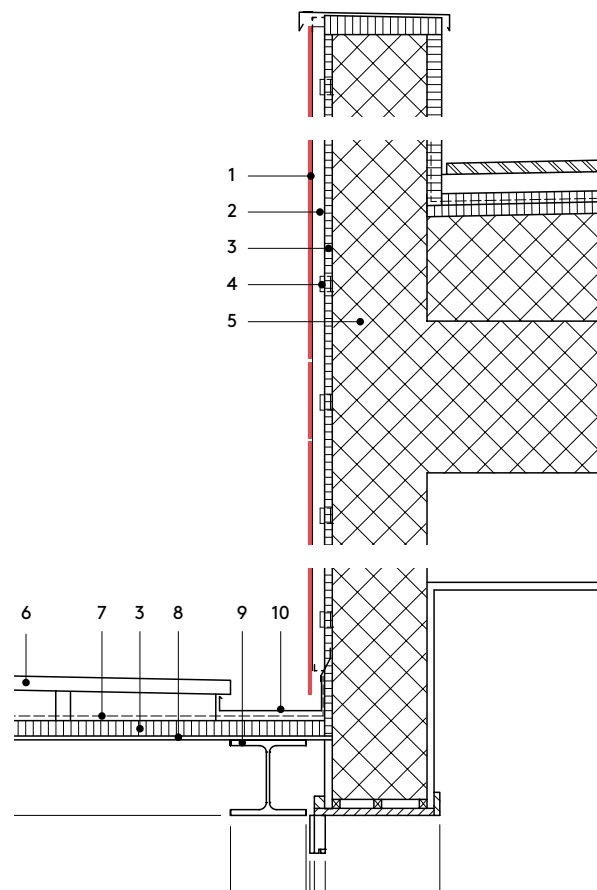
Vertical section 1:20
