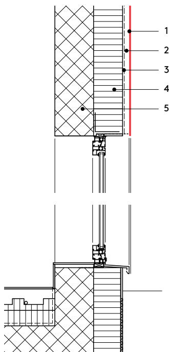
Vertical section 1:20
