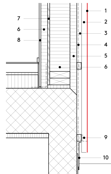
Vertical section 1:20
