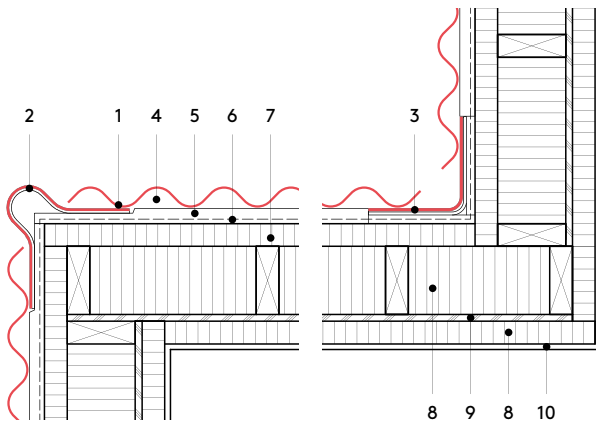
Horizontal section 1:20
