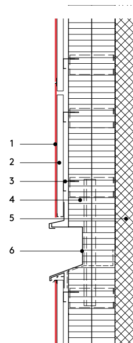
Vertical section 1:20
