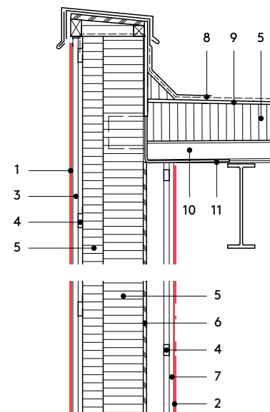
Vertical section 1:20
