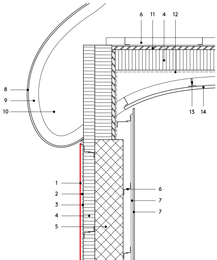
Vertical section 1:20
