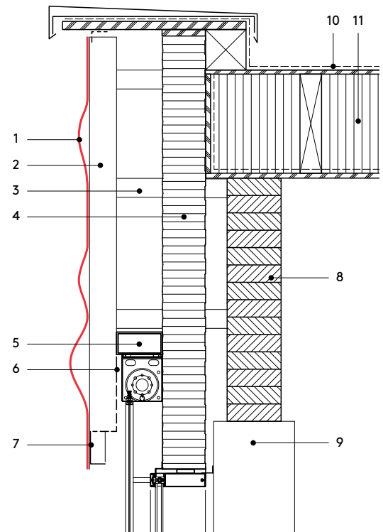
Vertical section 1:20
